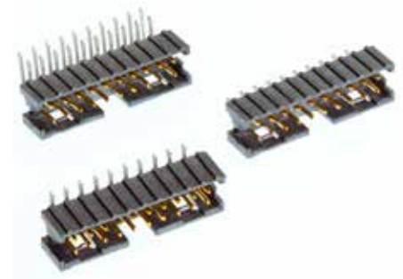
3M™ Shrouded Board Mount Header, 159 Series
