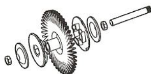
Brush Assembly
