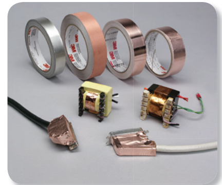
3M™ EMI Shielding Tapes prevent the emission of radio waves that can cause interference with electronic devices.
