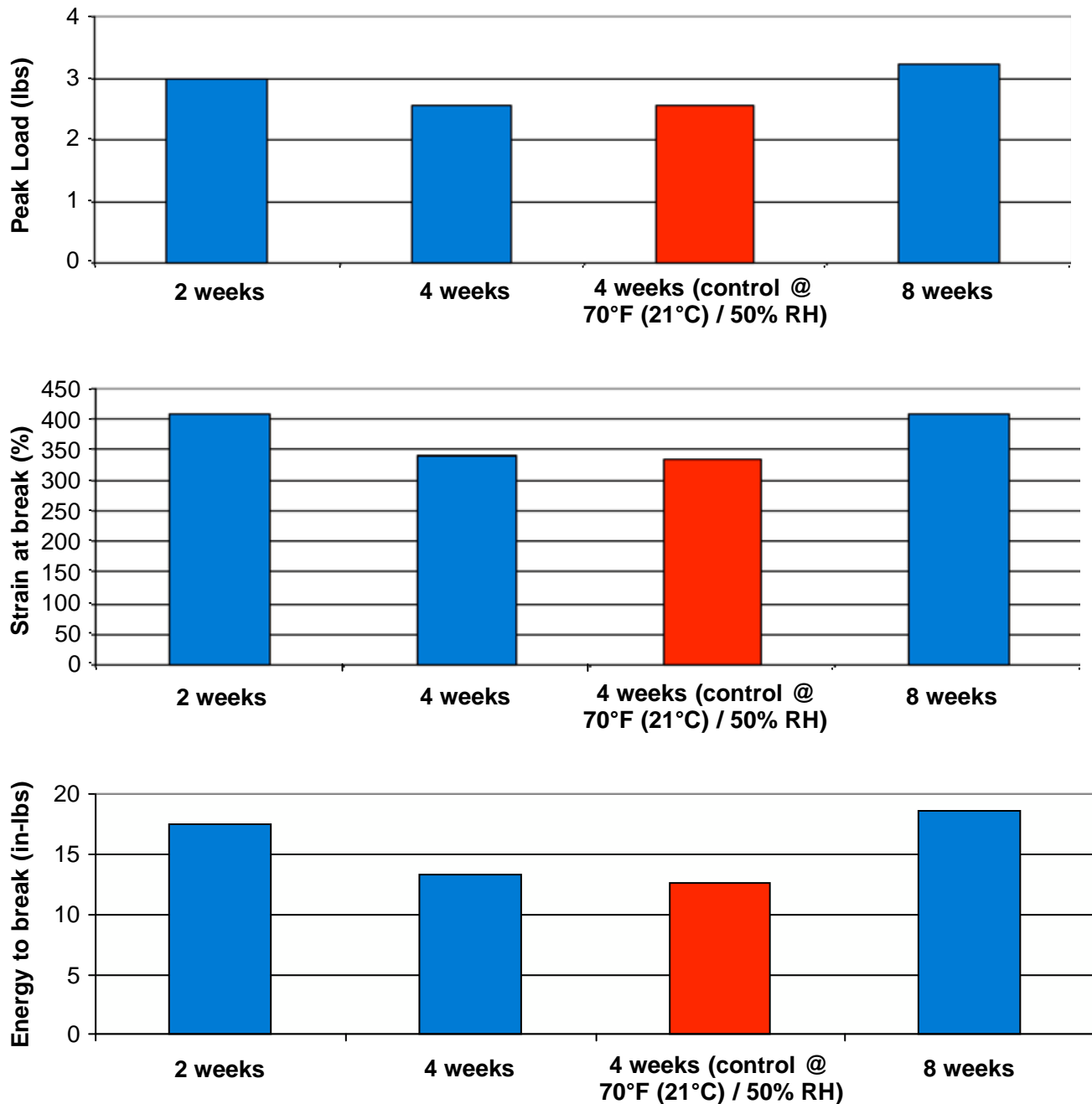
Chart #1 3M™ Extreme Sealing Tape 4412N – Tensile Strength Effects of high temperature & high humidity on ionomer film only Tensile testing on 1/2" wide ionomer film only Aged at 185°F (85°C) and 85% RH
