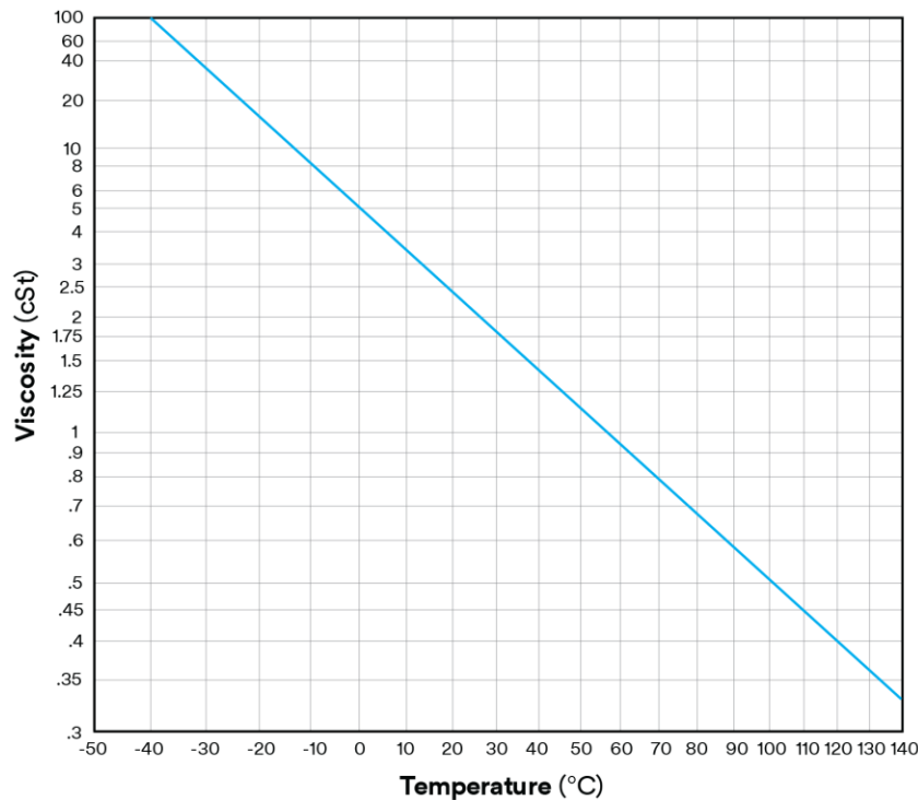
3M™ Fluorinert™ Electronic Liquid FC-70 Viscosity vs. Temperature
