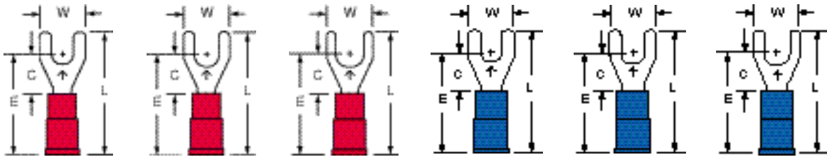
MVU18-6F MVU18-8F MVU18-10F MVU14-6F MVU14-8F MVU14-10F Stud Size 6 8 10 6 8 10 Wire Range 22-18 22-18 22-18 16-14 16-14 16-14
