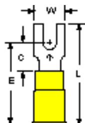
MV10-6FB 6 12-10
