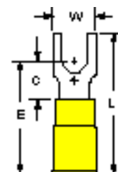
MV10-10FB 10 12-10
