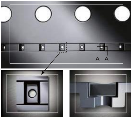
3M™ Polycarbonate Ultra Precision Carrier (UPC) 3000UB for 0603 (0201) package
