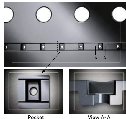
3M™ Polycarbonate Ultra Precision Carrier (UPC) 3000UP for 0603 (0201) package
