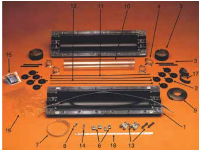
3M™ Pressurized Closure 51P Series
