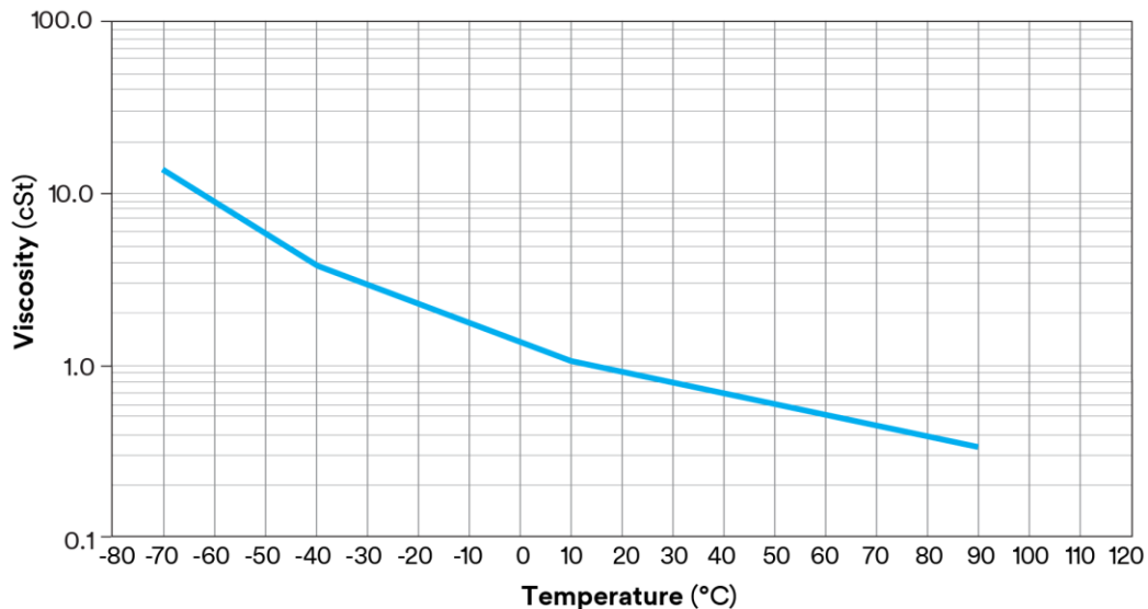
3M™ Fluorinert™ Electronic Liquid FC-770 Viscosity vs. Temperature
