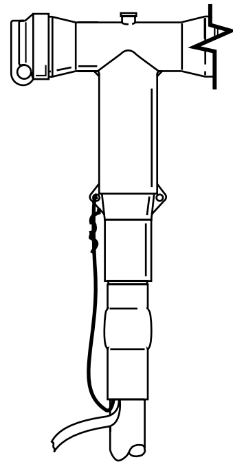
5815 Tee Module with Adapter Kit Installed
