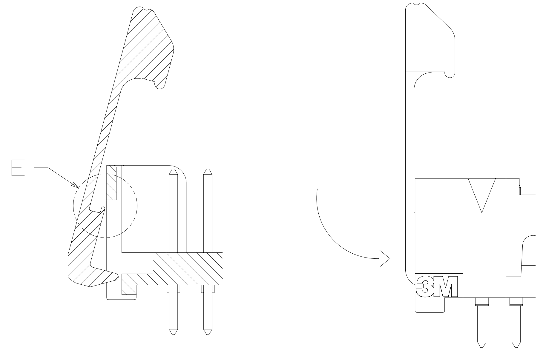
SECTION D - D SCALE 6x
