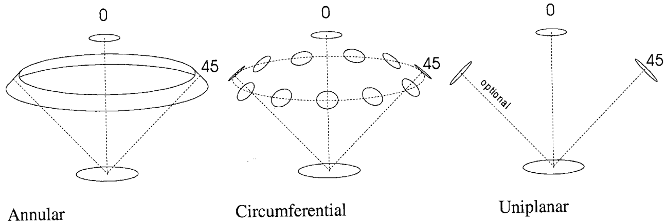
FIG. 1 Three Types of 0/45 (45/0) Instrument
