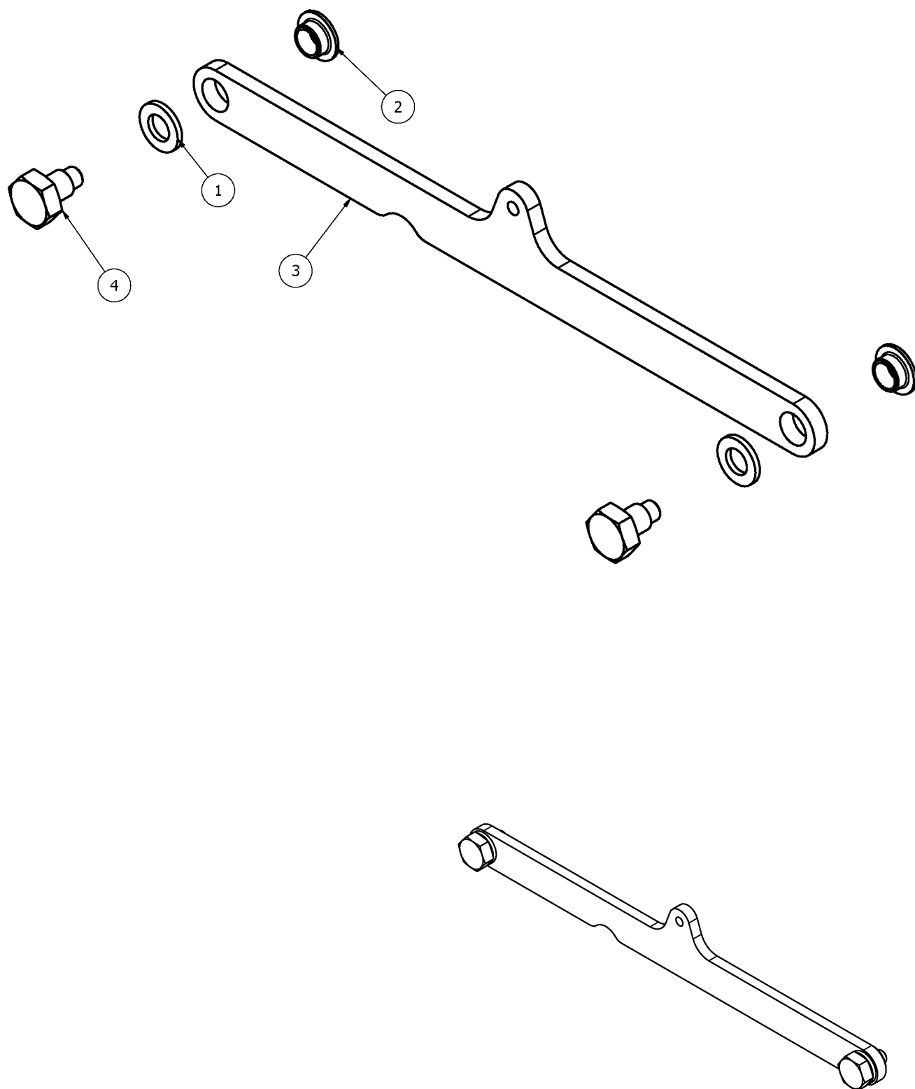
Figure 23079 – Upper and Lower Taping Head / Arm Assembly
