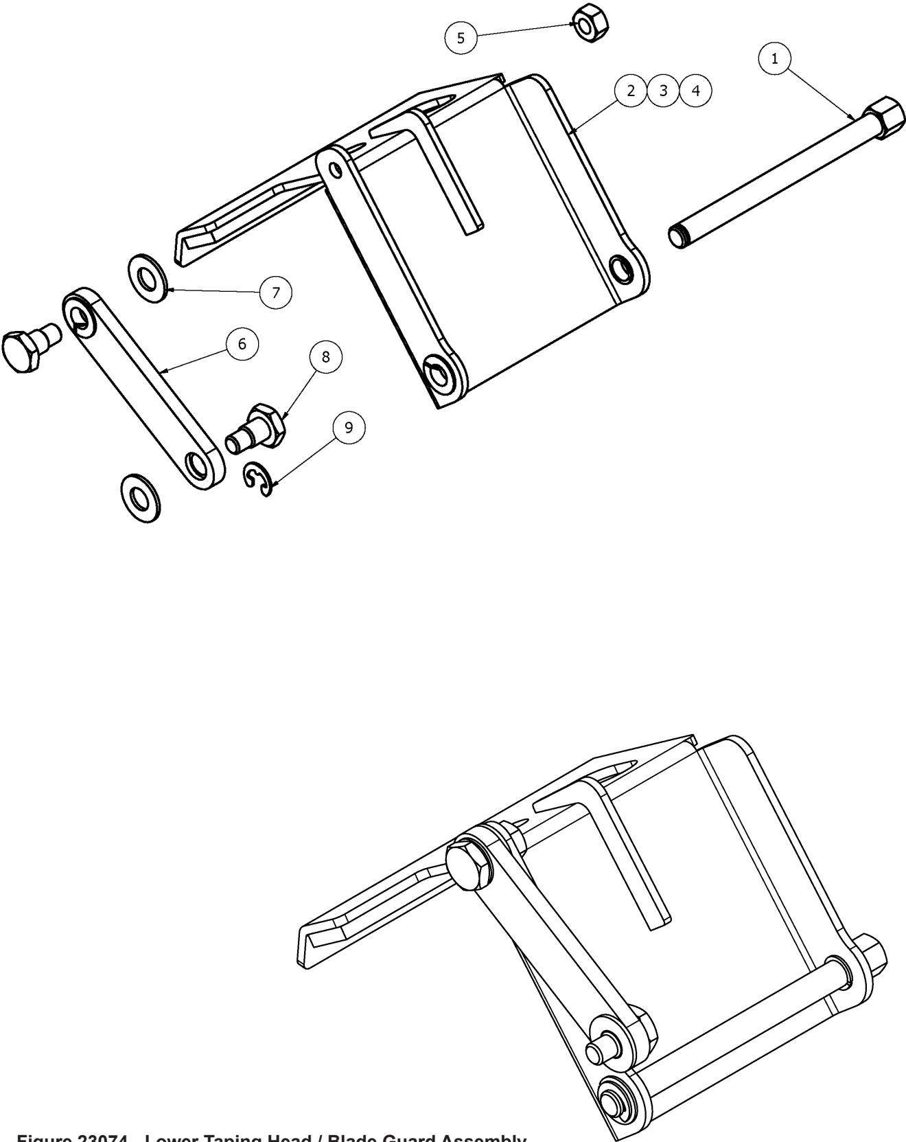
Figure 23074 - Lower Taping Head / Blade Guard Assembly
