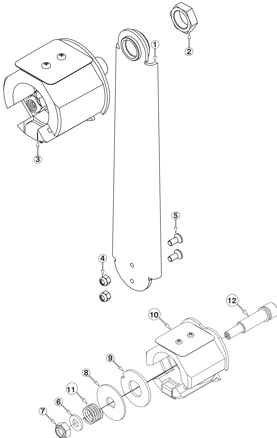
Figure 16103 - Upper and Lower Taping Head / Tape Drum/Arm Assembly
