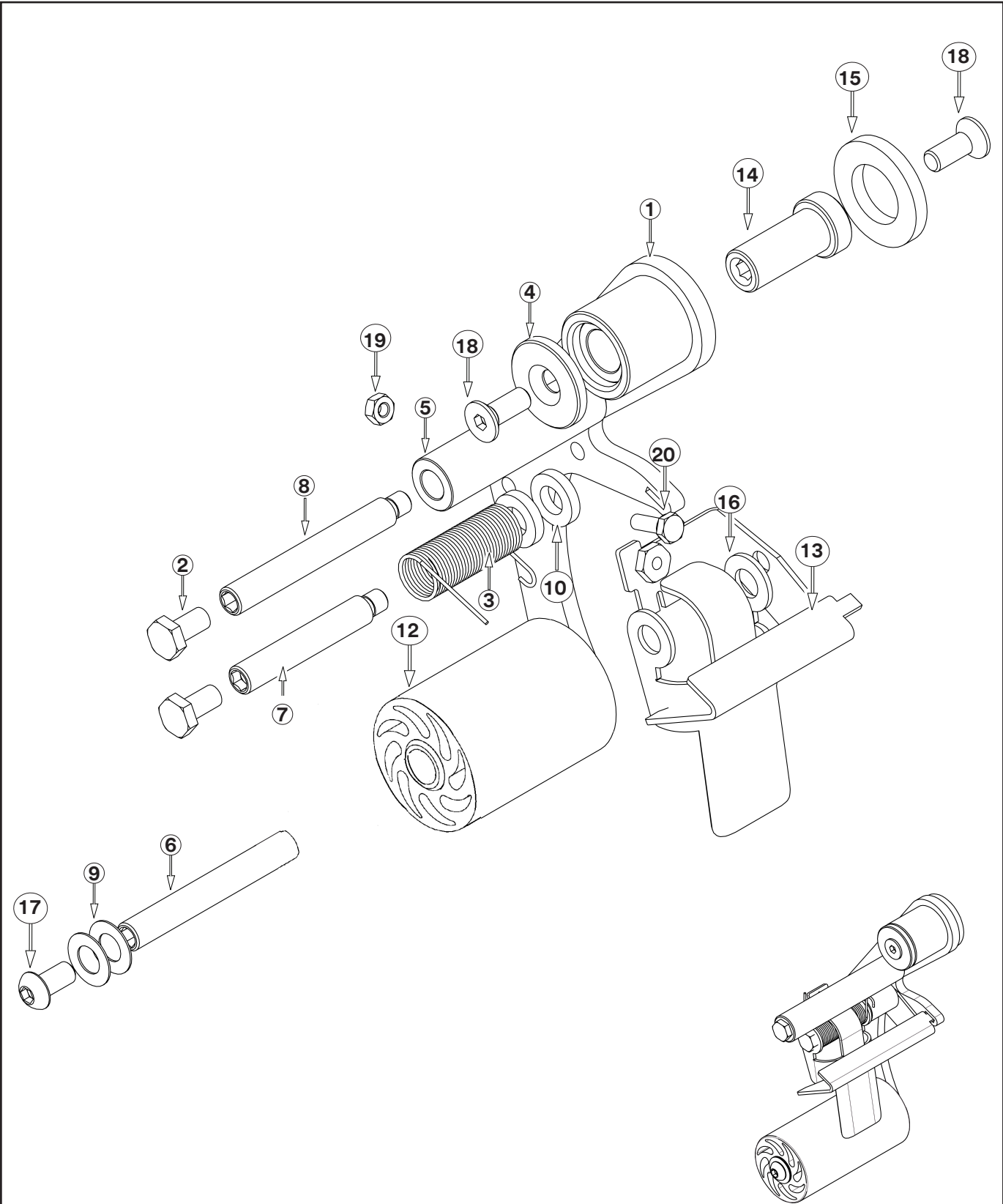
Figure 16100 - Taping Head / Applying Assembly
