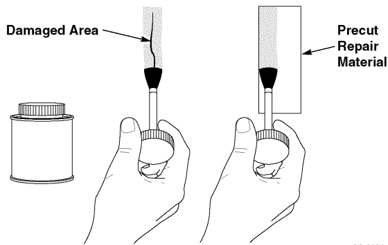
Figure 11. Apply Adhesive
