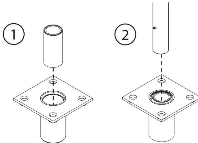
Figure 6 - Installing the Davit Base Adapter
