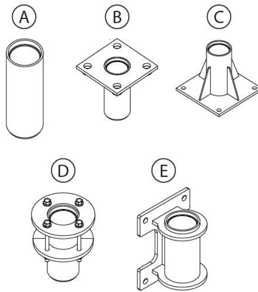
Figure 5 – bossoirs compatibles
