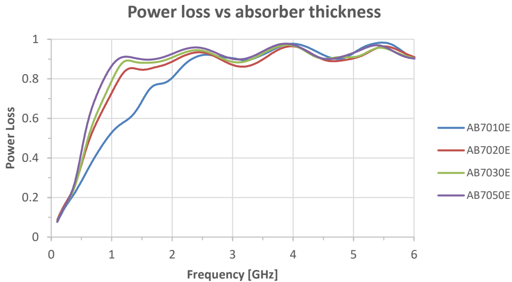
Figure 3. Transmission Attenuation Power Ratio
