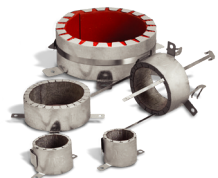
3M™ Fire Barrier Ultra Plastic Pipe Device
