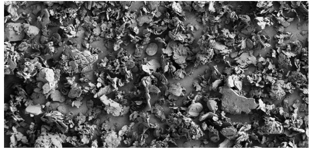
100 \mu m SEM micrograph: Grade CFA 75
