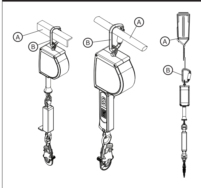
Figure 6 - Connecting to Anchorage
