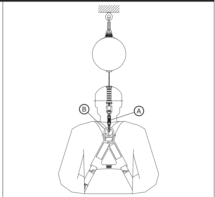
Figure 7 - Connecting to a Harness
