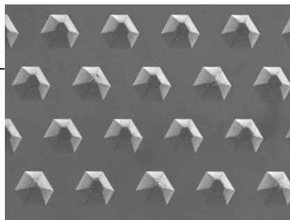
Scanning Electron Microscope (SEM) image of the 3M™ Trizact™ Pad Conditioner T Series B25T-2910 microreplicated surface
