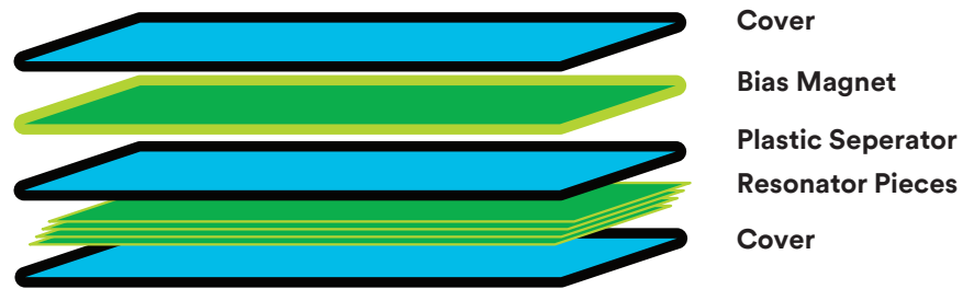
Figure 10: Prior art of magneto-mechanical resonator.
