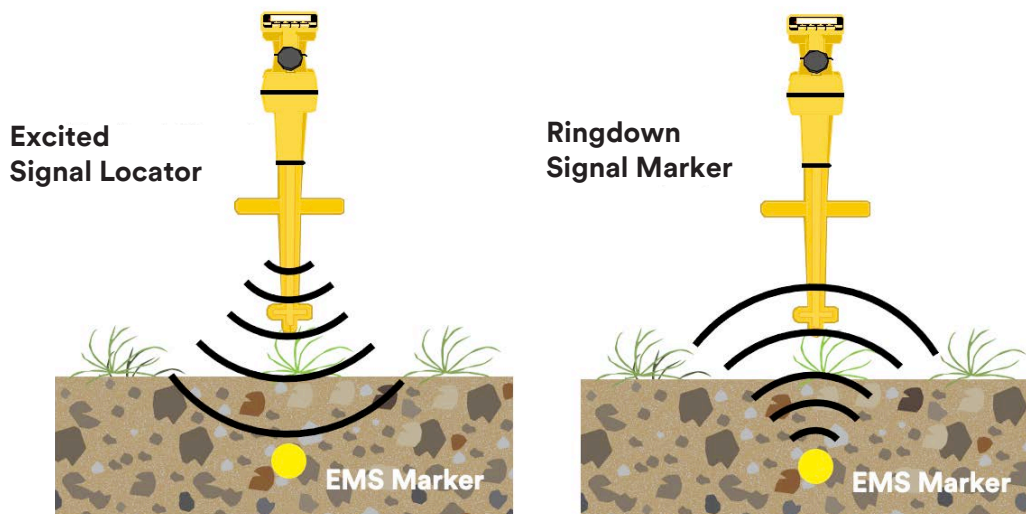
Figure 8: Locator to marker excitation and reflection.
