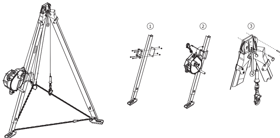
Figure 9 - Tripod Mounting
