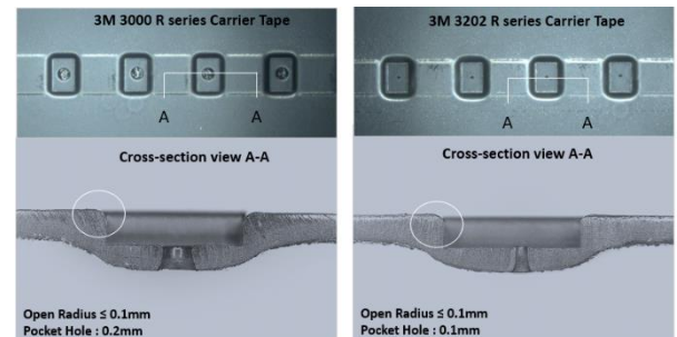
3M™ Polycarbonate Carrier 3000UPR or 3000UBR, 8mm with improved pocket opening radius with 0.2mm pocket hole
