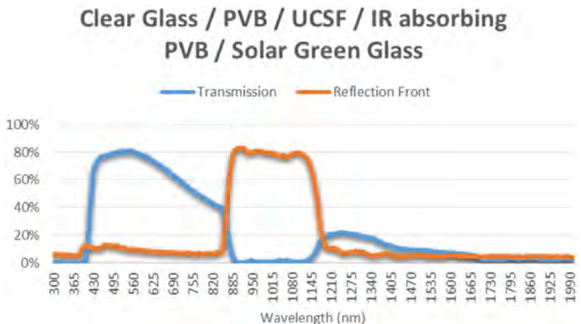
FIGURE 6 Dramatic reductions in infrared (IR) heat (achieved by IR rejection films configured with IR-absorbing polyvinyl butryl [PVB]) minimizes solar energy impact on picture generating units (PGUs); this configuration also increases cabin comfort and reduces demand on air conditioning (AC) units
