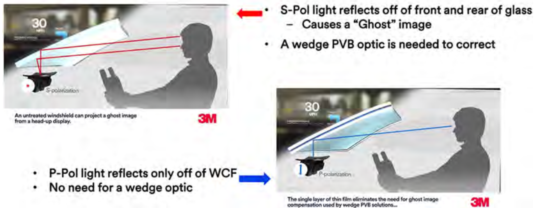
FIGURE 3 Windshield combiner film (WCF) eliminates the need for polyvinyl butryl (PVB) wedges to correct ghosting artifacts
