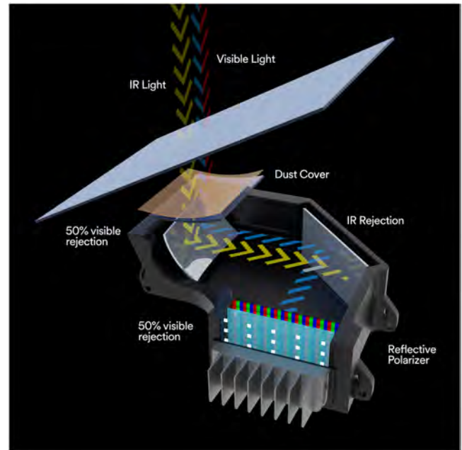
FIGURE 8 Integrating a reflective polarizer into the picture generating unit (PGU) dust cover can reduce visible light (and solar heat) infiltration by approximately 50%. IR, infrared
