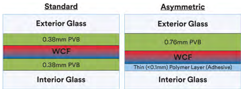
FIGURE 5 Glazing options with combiner film: asymmetrical adhesive layers retains safety and durability while improving visual quality. PVB, polyvinyl butryl ; WCF, windshield combiner film
