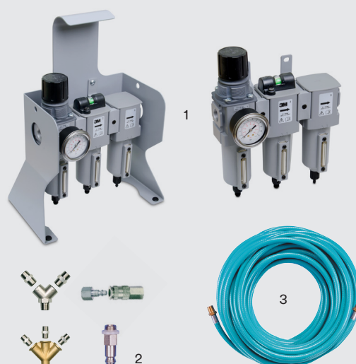
1. 3M™ Aircare™ Filtration Units (wall-mounted or stand alone)
