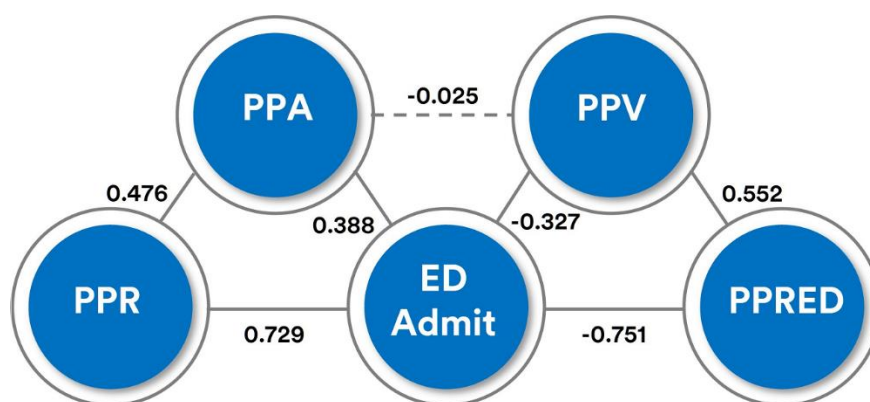
Figure 1: Correlation of \%(A-E)/E for PPAs, PPVs, PPRs, PPREDs and ED Admit. Dashed line indicates the correlation is not significant at the 0.01 level
