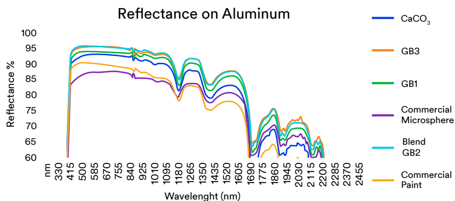
Figure 4 – Cumulative solar reflectance spectral curves.
