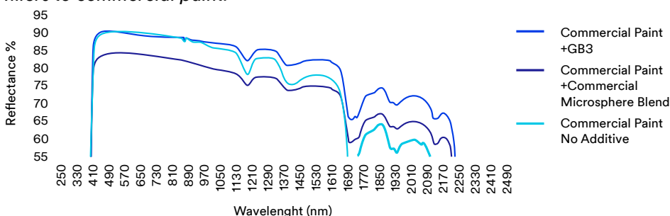
Figure 8 – Cumulative solar reflectance spectral curves for post addition of fillers to commercial paint.
