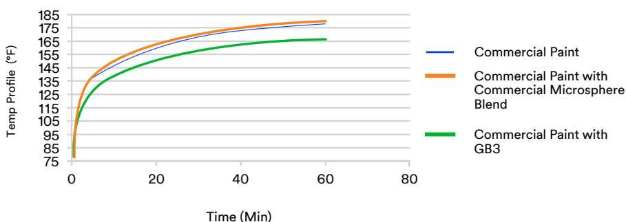
Figure 7 – IR heat lamp test result for post addition of fillers to commercial paint.
