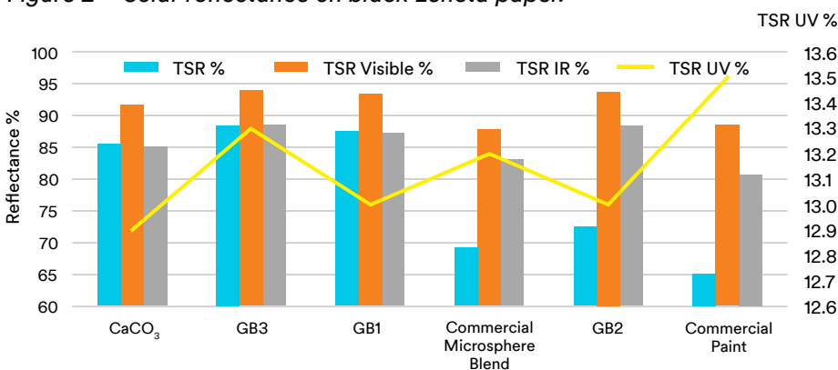
Figure 2 – Solar reflectance on black Leneta paper.
