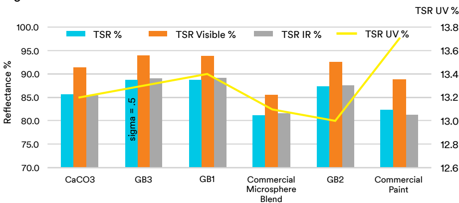
Figure 3 – Solar reflectance on 3003 aluminum.
