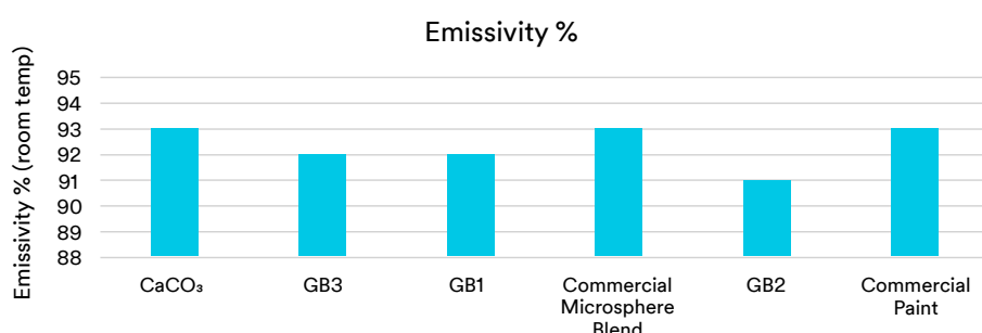
Figure 5 – Emissivity test results
