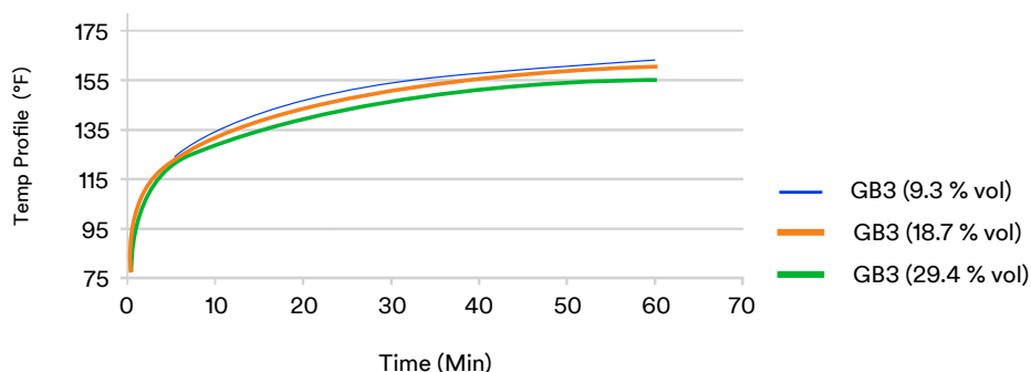
Figure 6 – IR heat lamp test curves for Glass Bubbles 3.
