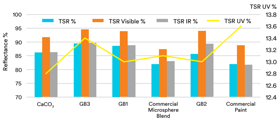
Figure 1 – Solar reflectance on white Leneta paper.
