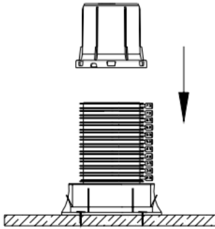
Position CID and line up slot and arrow on height adjuster with tab on CID
