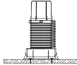
Snap height adjuster onto CID
