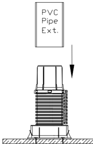
PVC extension for concrete greater than 12 in. thick.
