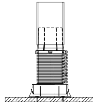
CID with height adjuster and PVC extension ready for 16 inch concrete pour
