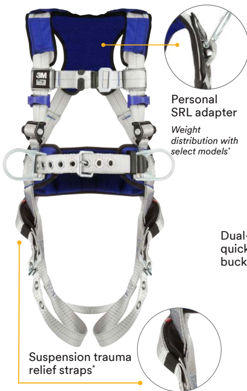
3M™ DBI-SALA® ExoFit™ X100 Harness
