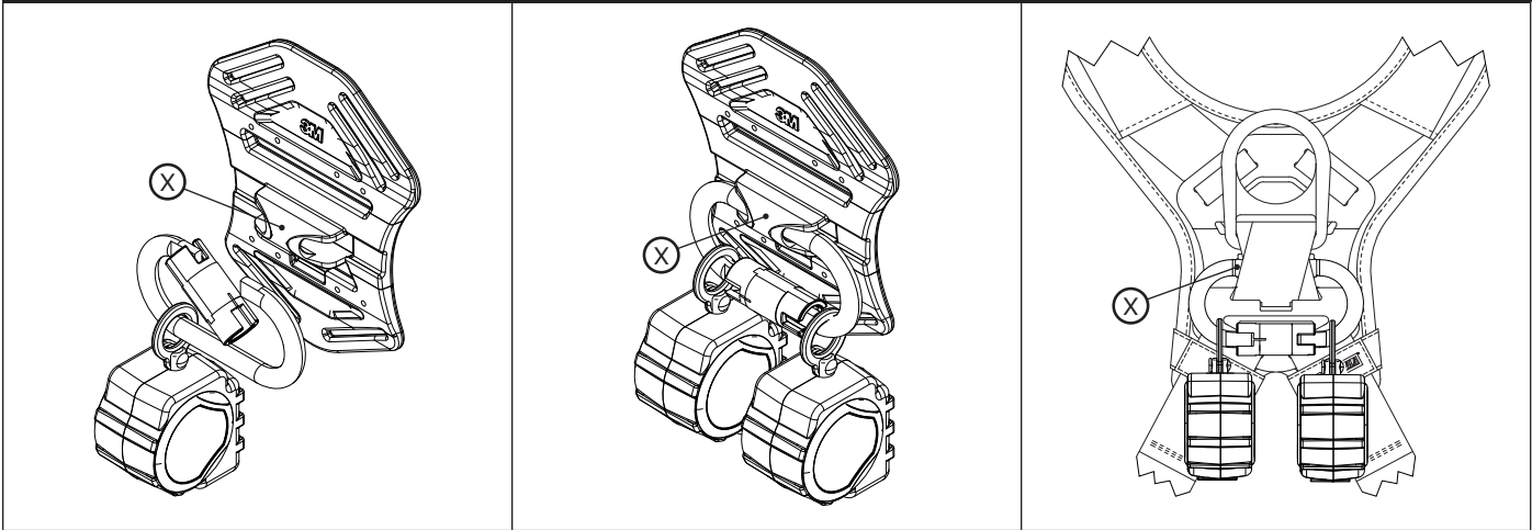
Figure 13 - SRD Adapter
