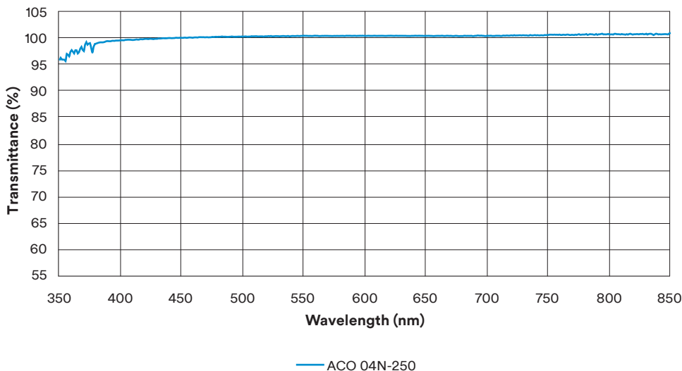
Transmission vs. Wavelength (Corrected for Reflection Loss of LCD) for 3M ACO 04N-XXX on Glass
