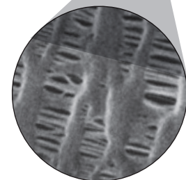
Hydrophobic membrane with pores approx. 0.03 \mu\text{m}
