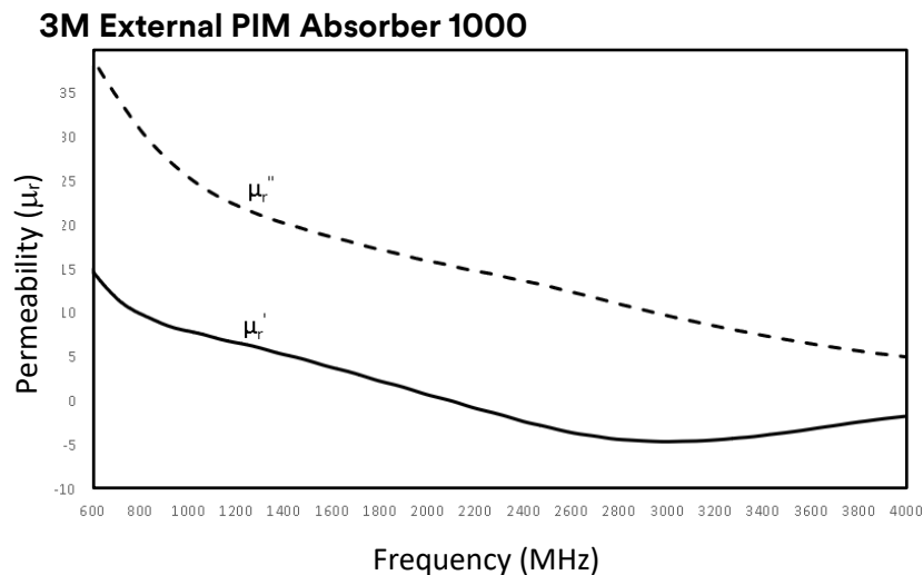
Figure 1. Real and Imaginary Part of Permeability with Frequency
