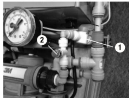
1 - blend line shutoff valve 2 - blending valve
