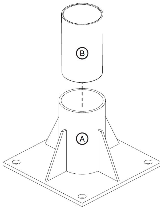
Figure 2 - Composants
