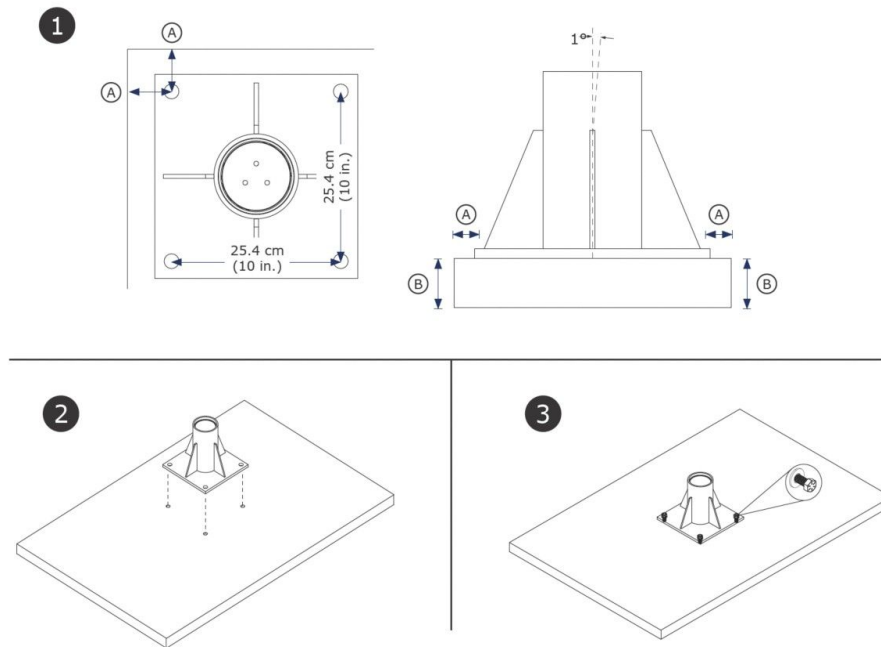
Figure 5 - Installing the Floor Mount Base
