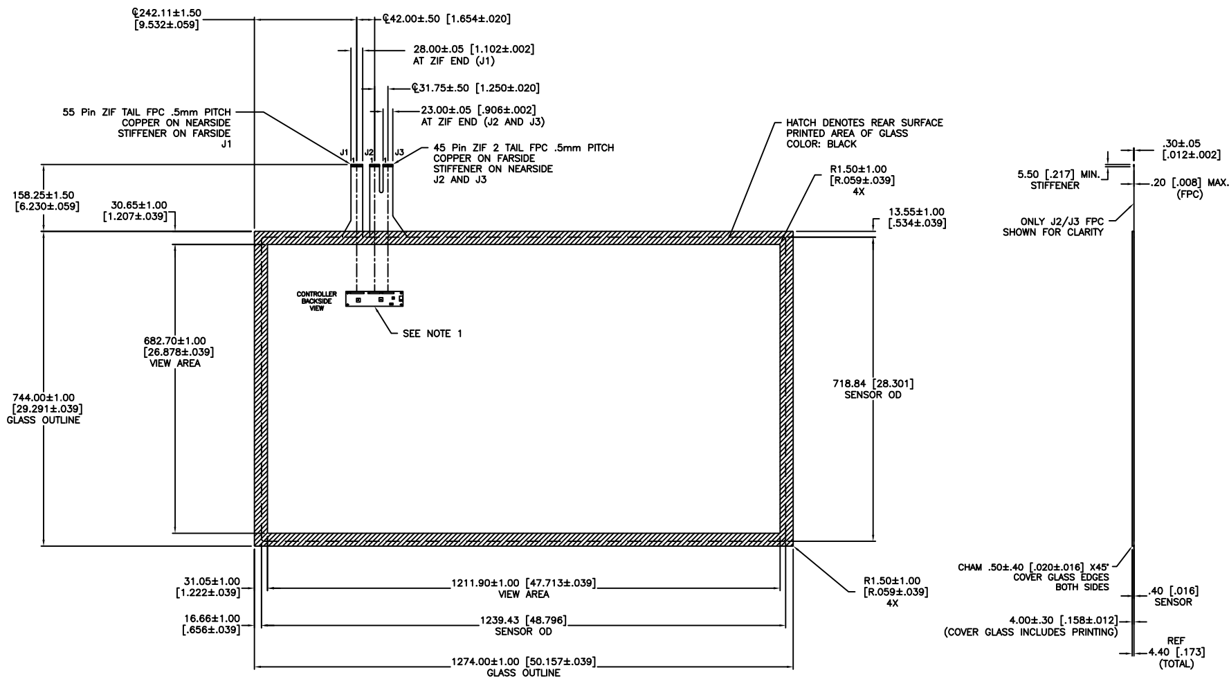
SENSOR FRONT
