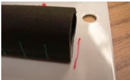
Creep of seal: seal has crept back about 2 mm from original position (indicated by red line)
