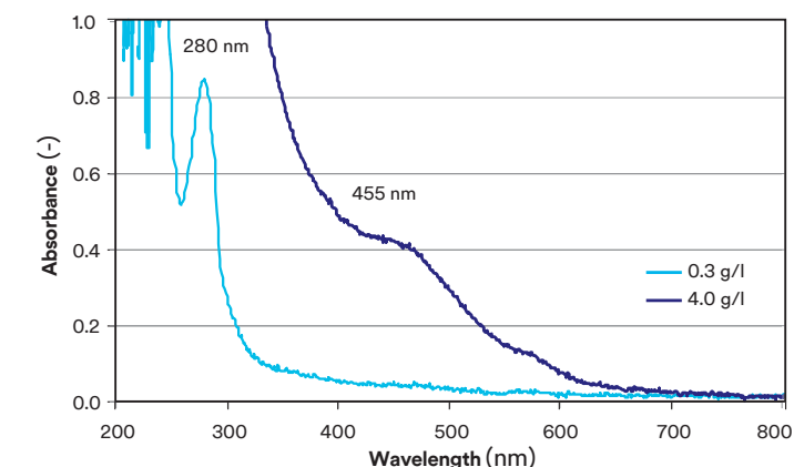
Figure 2: UV-Vis spectrum of “synthetic red wine” (two different concentrations, cuvette thickness 1 cm).
