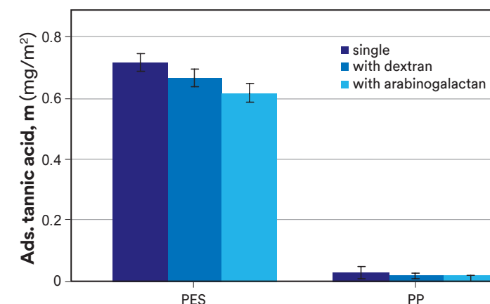
Figure 4. Adsorption of tannic acid (0.1 g/L) from single solute solution and mixtures with arabinogalactan or dextran (1 g/L; in "synthetic wine") to PES and PP membranes (#1 and #2), relative to the membrane specific surface area.
