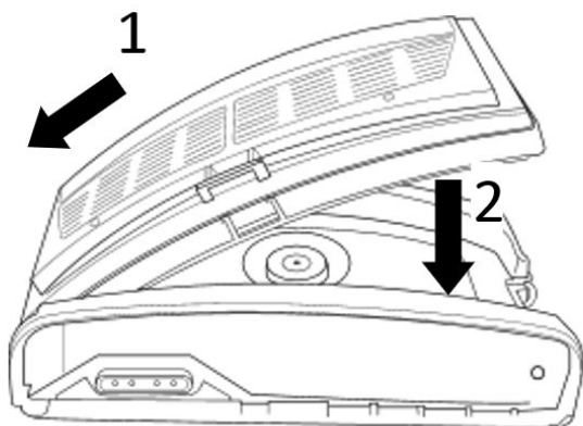
Figure 2: Fig. 4 – Attaching filter/cartridge to blower
