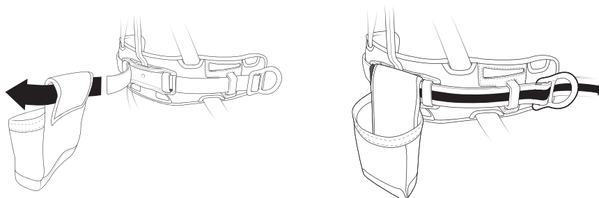
Figure 15 - Tool Bag Attachment
