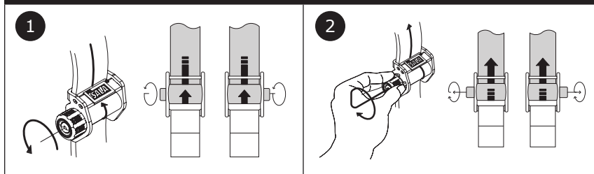
Figure 9 - Revolver Adjusters
