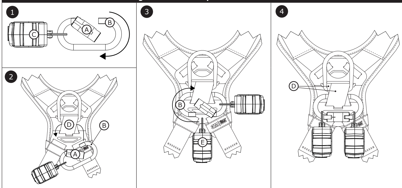
Figure 10B – Mousqueton d'interface
