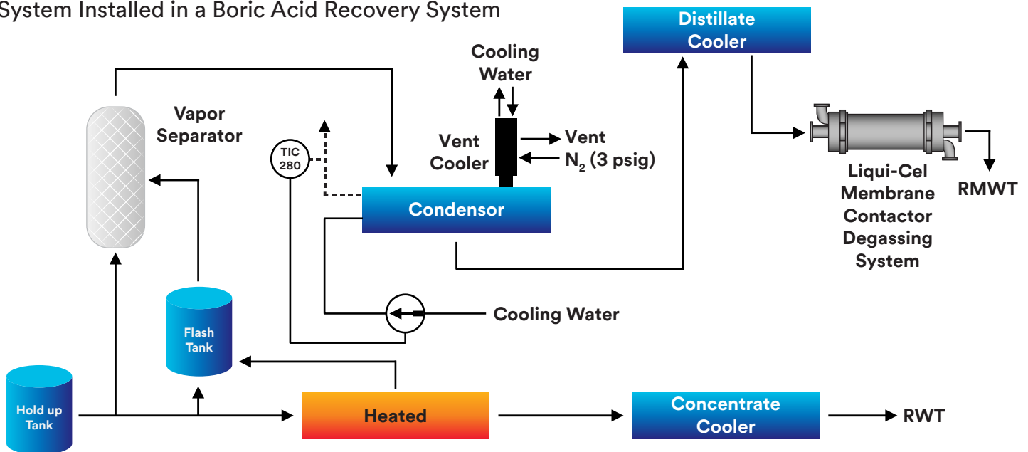
Figure 1. System Diagram with 3M™ Liqui-Cel™ Degassing System Installed in a Boric Acid Recovery System
