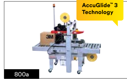
800a 3M-Matic™ Side Belt Adjustable Case Sealer 800a is an adjustable side belt drive case sealer. Seals up to 40 cases per minute, using tape widths from 36mm to 48mm, and also 72mm tape.
