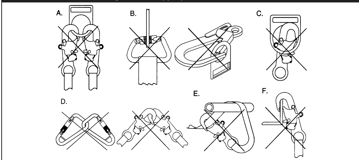
Figure 5 - Inappropriate Connections
