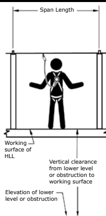
Figure 10 - Fall Clearance for Self Retracting Lifelines
