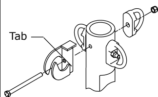
Figure 12 - Assembly
