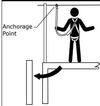
Figure 3 - Swing Fall
