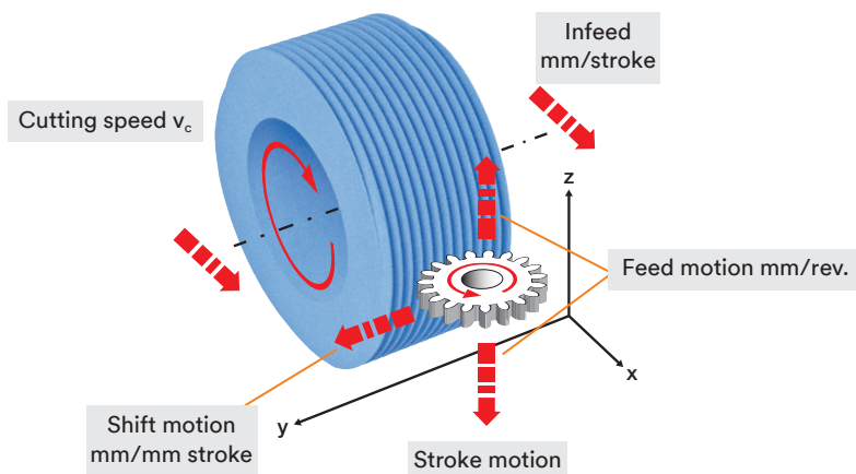
3M™ Cubitron™ II grinding worm movement
