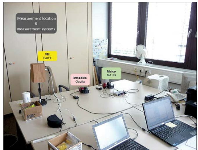
Figure 4 Experimental setup of the second study. Each measurement system is controlled by a separate computer.
