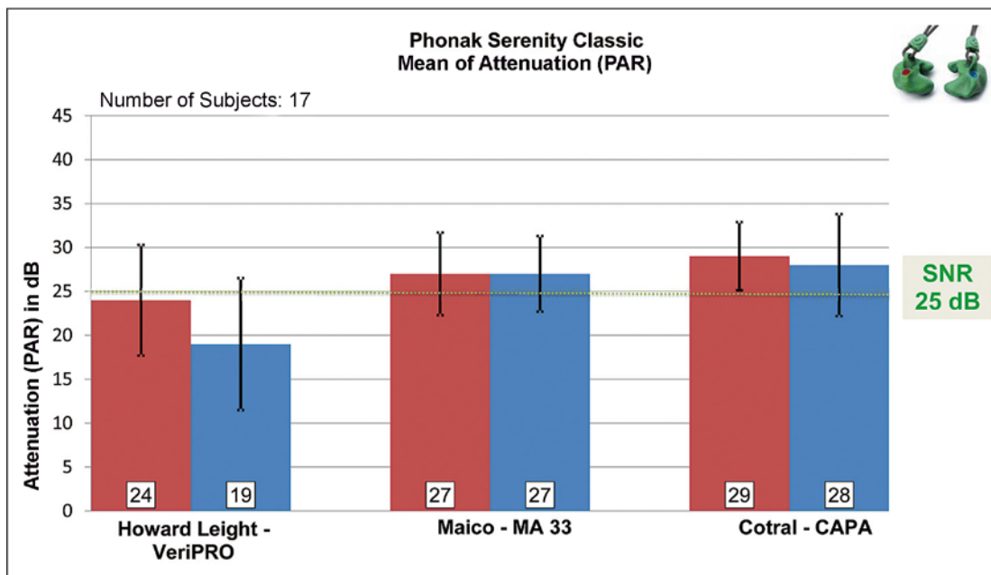
Figure 8 Comparison of PAR values for the custom molded earplug Phonak Serenity Classic (mean values and standard deviations for 17 subjects), obtained with the measurement systems VeriPRO, MA 33 and CAPA.
