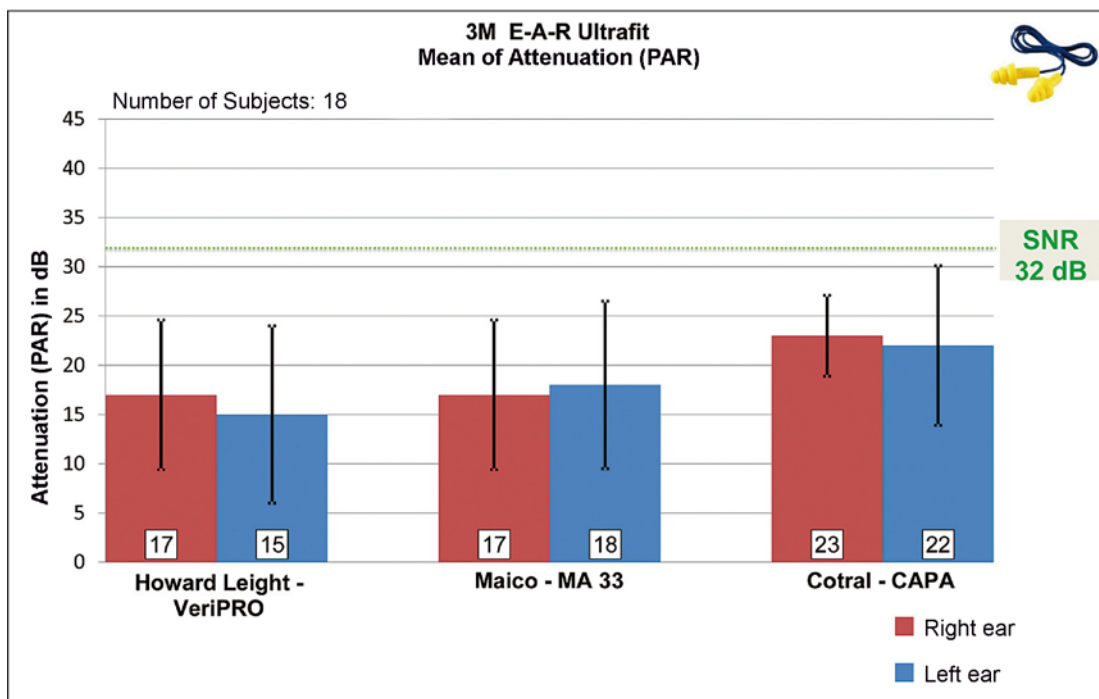
Figure 9 Comparison of PAR values for the premolded earplug 3M E-A-R Ultrafit (mean values and standard deviations for 18 subjects), obtained with the measurement systems VeriPRO, MA 33 and CAPA.
