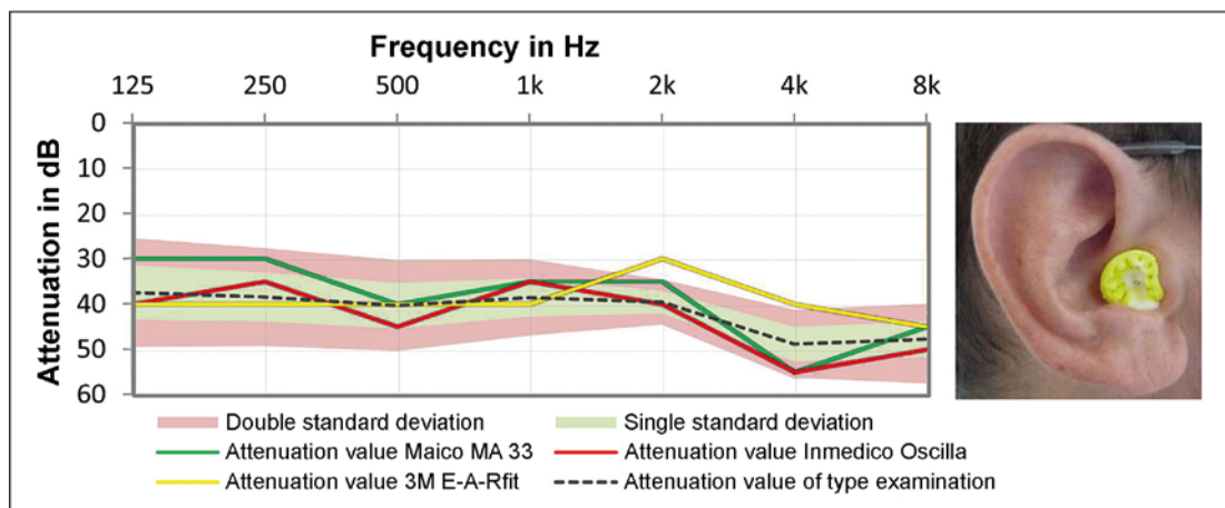
Figure 16 Comparison of the individually determined attenuation values for a subject (right ear) with the values of the type examination test in the frequency range of 125 Hz to 8 kHz for the 3M E-A-RSoft FX. The colored areas include mean \pm 1 \times standard deviation (light green) and mean \pm 2 \times standard deviation (pink). The individually determined curves agree well with the values of the type examination test.
