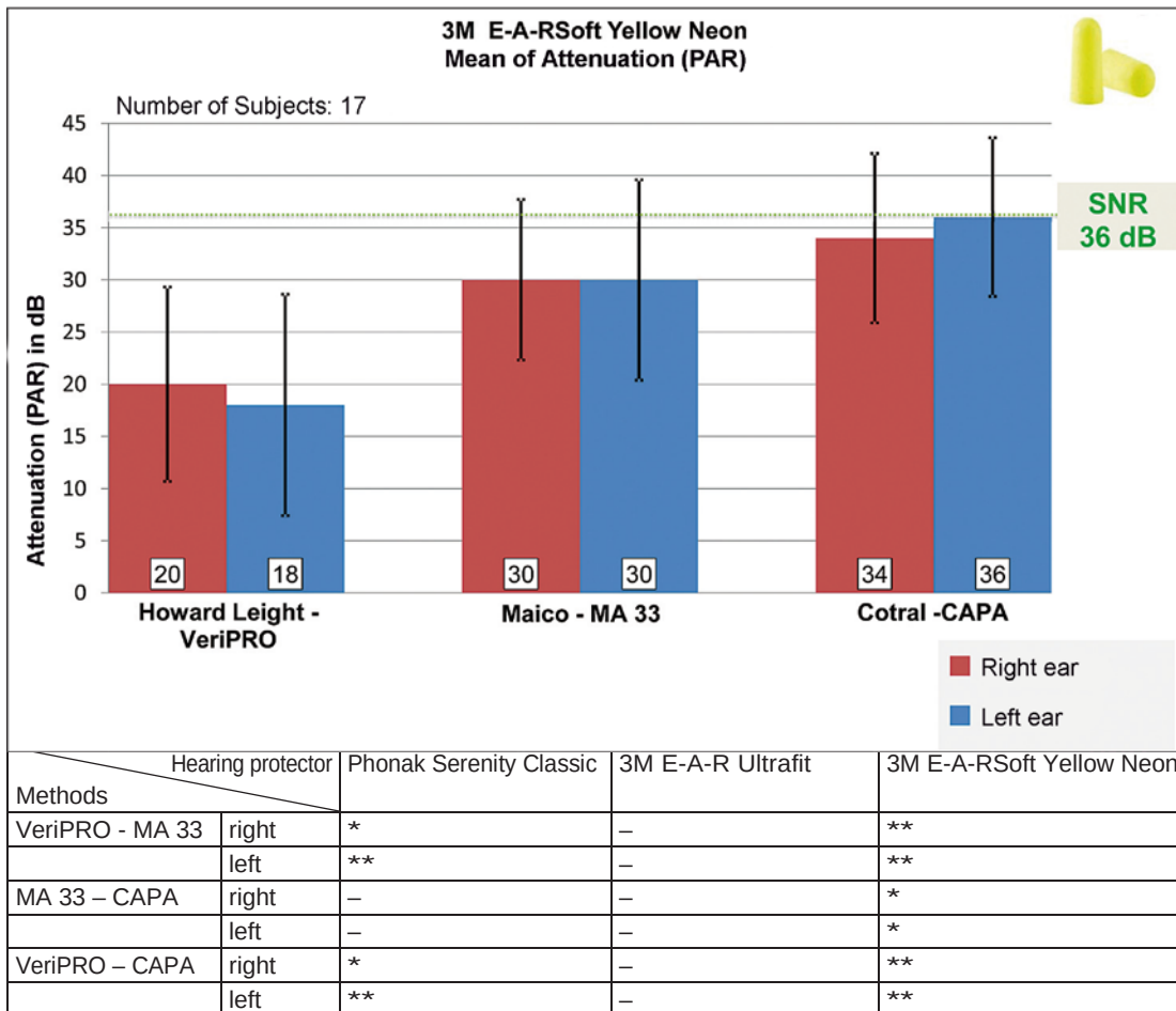
Figure 10 Comparison of PAR values for the foam earplug 3M E-A-RSoft Yellow Neon (mean values and standard deviations for 17 subjects), obtained with the measurement systems VeriPRO, MA 33 and CAPA.
