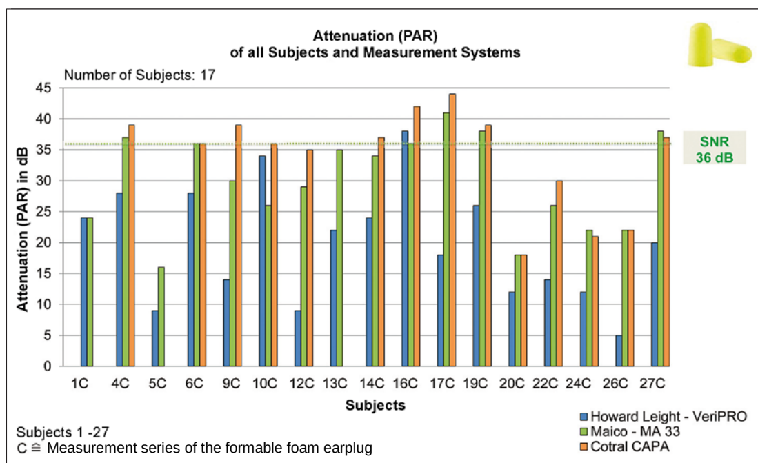
Figure 13: PAR-values for the individual subjects and the three measurement methods VeriPRO, MA 33 and CAPA (mean values and standard deviations in Figure 10).
