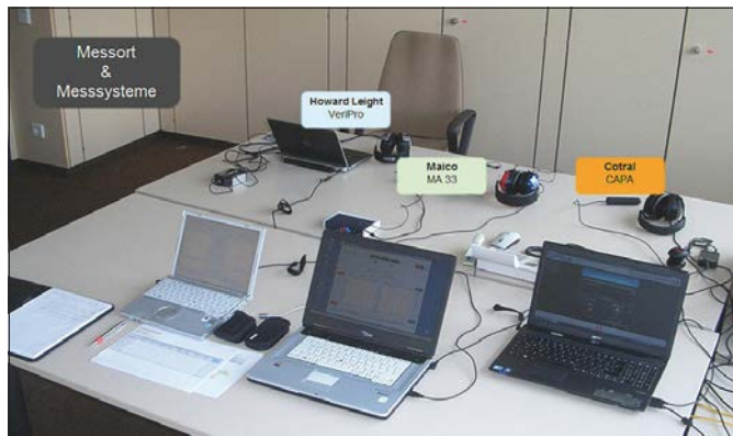
Figure 2 Experimental setup of first study. Each measurement system is controlled by a separate computer.
