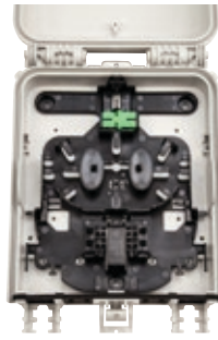
Inside of the 3M™ Fiber Network Interface Device NID-FO-1724-AT
